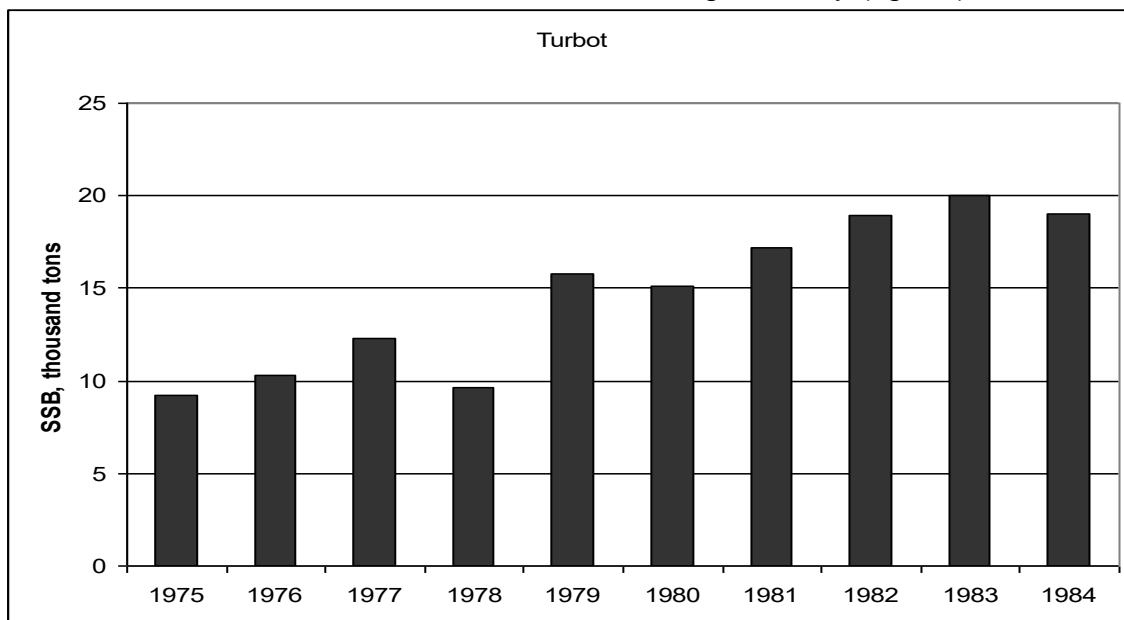
Fig. 10 – SSB s of the Black Sea turbot using the VPA method in modification of Babayan (from Efimov et al, 1989)
