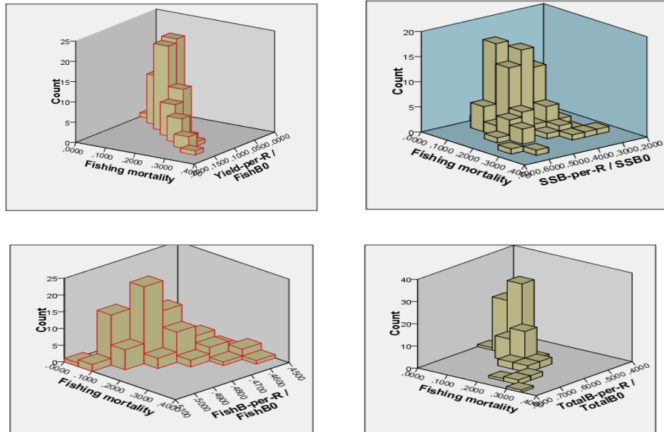
Fig 40 – Candidate F_{0.x} criterion estimation related to parameters of the stock in relative terms
