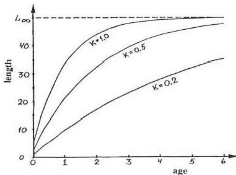
Fig 3 – A family of growth curves with different curvature parameters, different K values
