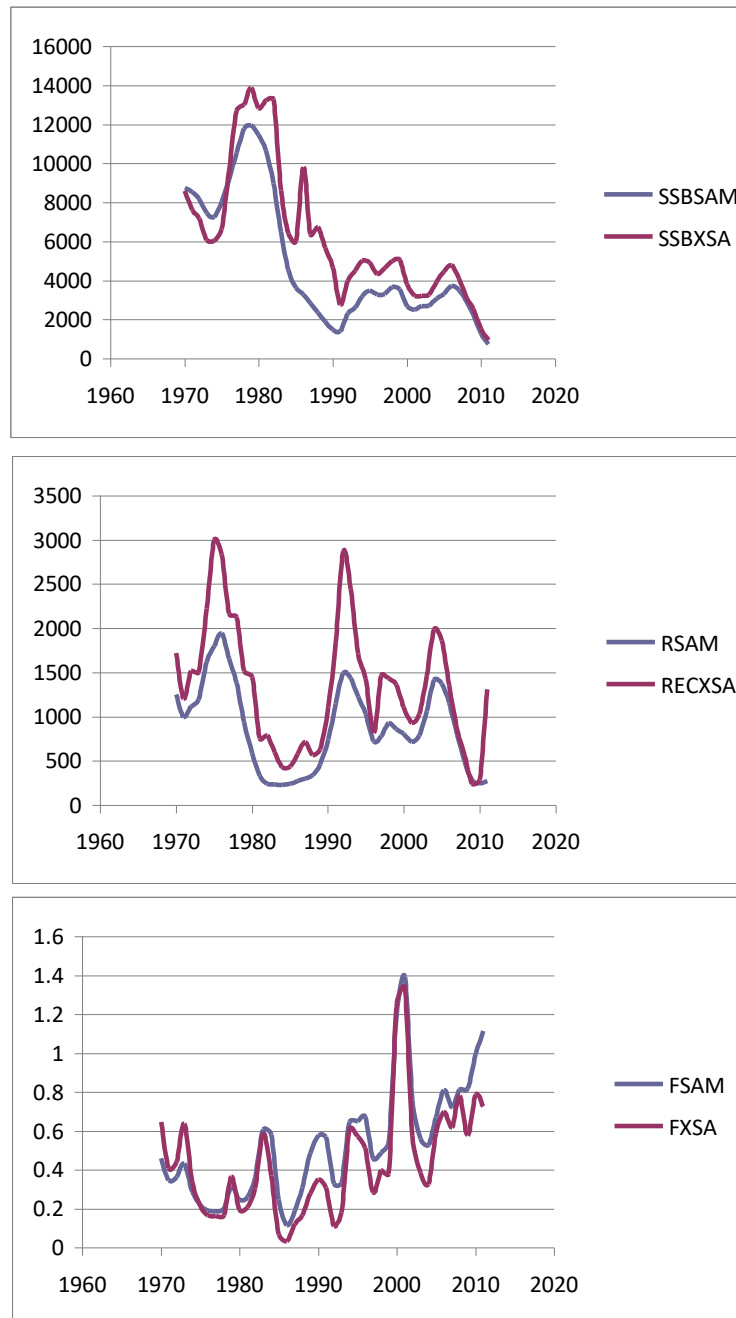
Fig. 32 – Trends in SSB, recruitment and fishing mortality according to SAM model and XSA.
