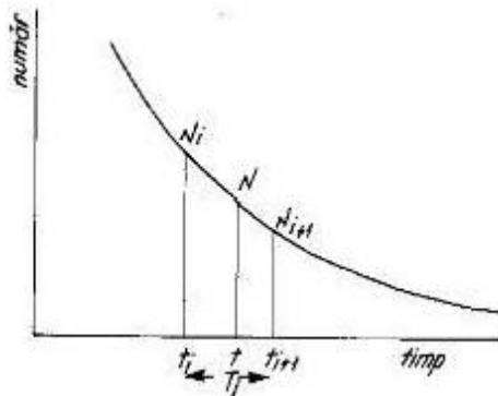
Fig 2 – Evolution of N in the interval T_i
