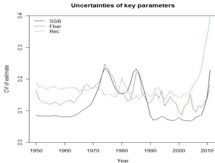
Fig. 34 – Uncertainties of key parameters
