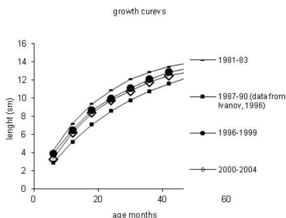
Fig 4 – Growth curves for the average cohorts of sprat for the periods: 1981- 83 (data from L. Ivanov, 1996), 1987-1990 (data from L. Ivanov, 1996), 1996-1999 (Daskalov)
