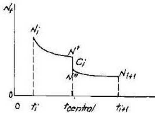
Fig 10 – Number of survivors during the interval T_i = t_{i+1} - t_i , capture extracted in the center of the interval (FAO, 2003)
