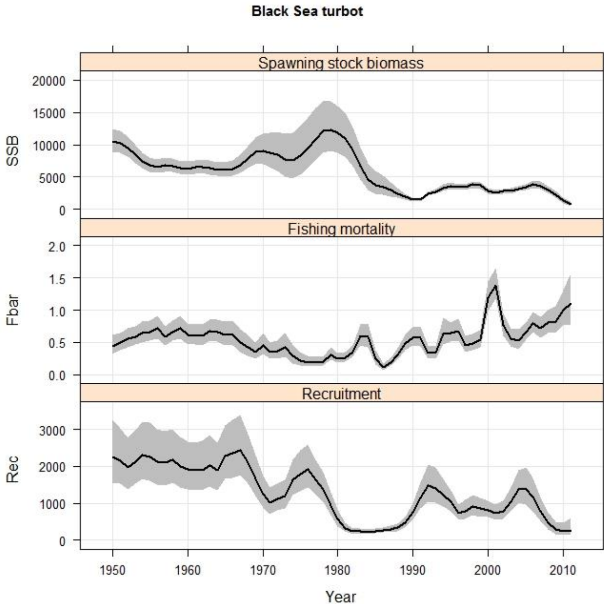
Fig. 33 – Time-series of turbot population estimates of total stock in the Black Sea (SAM model) including estimated IUU catches: recruitment, SSB and average fishing mortality (ages 4–8) with estimate of uncertainty.
