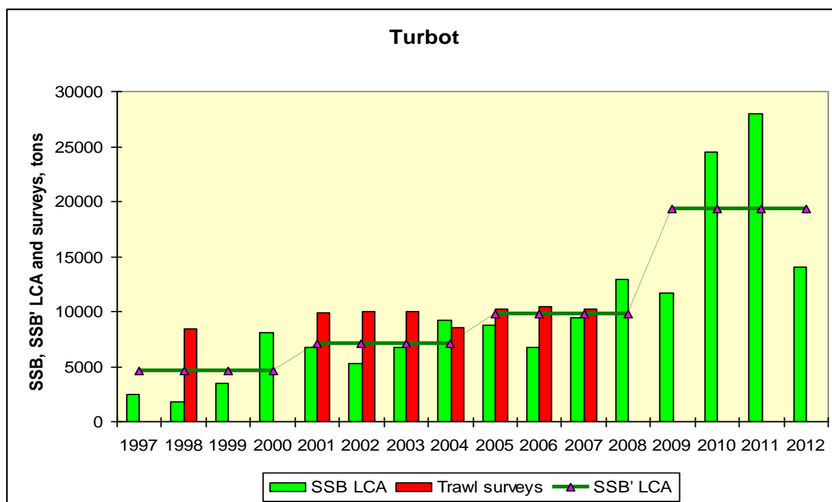
Fig. 27 – Turbot stock assessment in Ukrainian sector of the Black Sea using Jones cohort analysis method: SSB – without averaging by years of fishery (green columns), SSB' – with averaging the input data by 4-years periods (horizontal segments). Red columns – stock by the trawl survey data (after Shlyakhov et al, 2012b).
