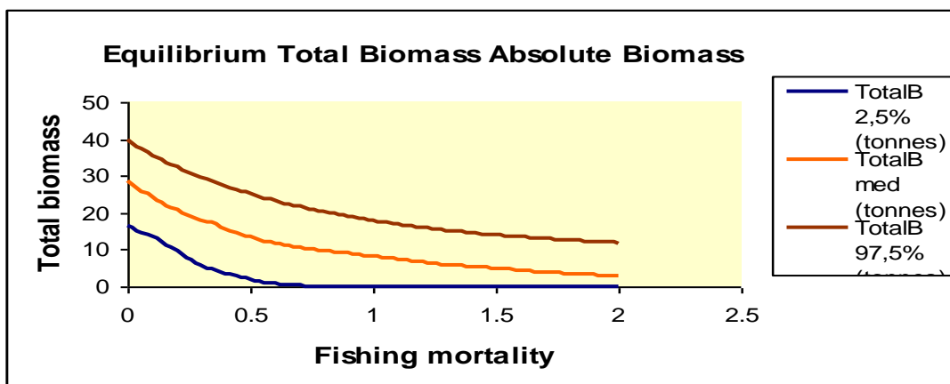
Fig 36 – Graphical representation of the equilibrium levels of exploitation with the corresponding CI.
