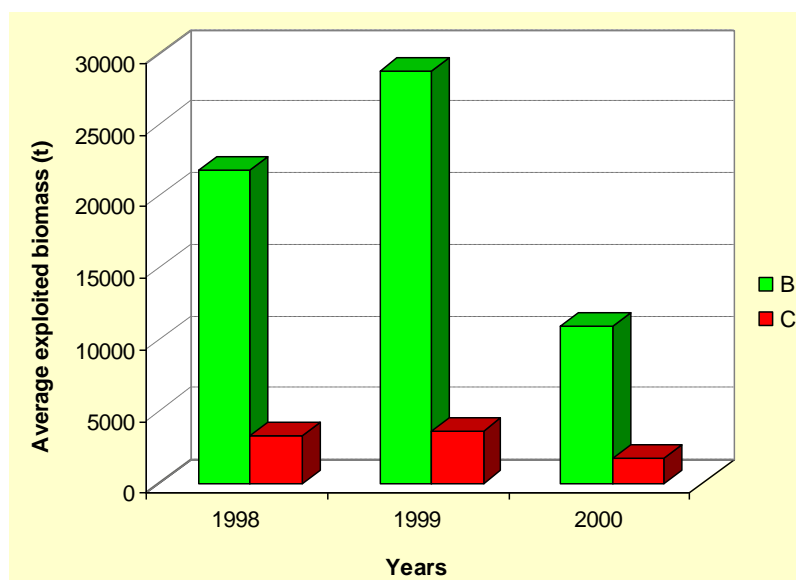
Fig 14 – Bulgarian sprat catches in the Black Sea and average exploited biomasses in 1998, 1999 and 2000 under LCA
