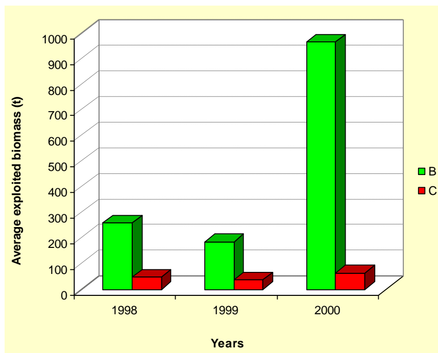
Fig 15 – Bulgarian anchovy catches in the Black Sea and average exploited biomasses in 1998, 1999 and 2000 under LCA
