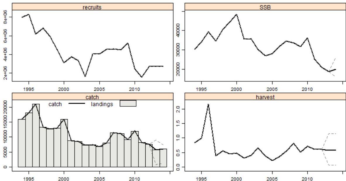
Fig. 30 – Historic trends and short term prediction (status quo) of relevant whiting stock parameters
