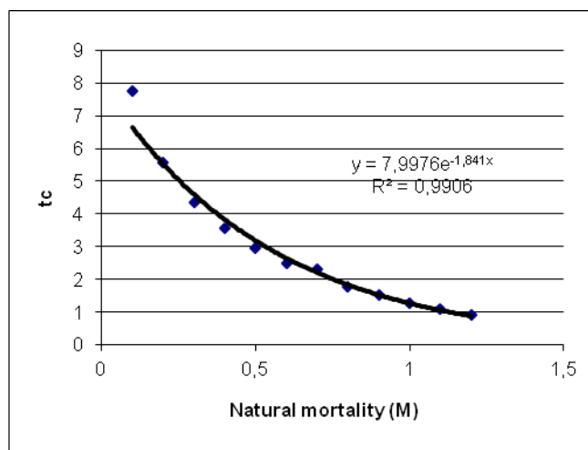
Fig 5 – Optimal exploitation age vs. instantaneous rate of natural mortality estimated by Kutty and Quasim (1965) method for Horse mackerel (2003-2005) in Bulgarian Black Sea territorial waters
