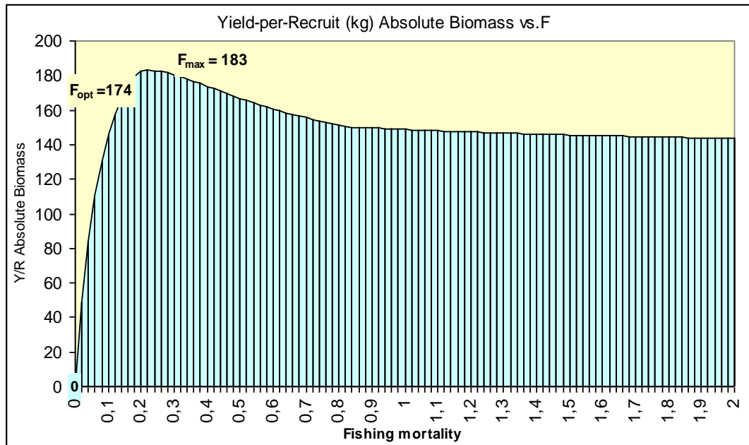
Fig 37 – Reference levels of turbot fishing mortality
