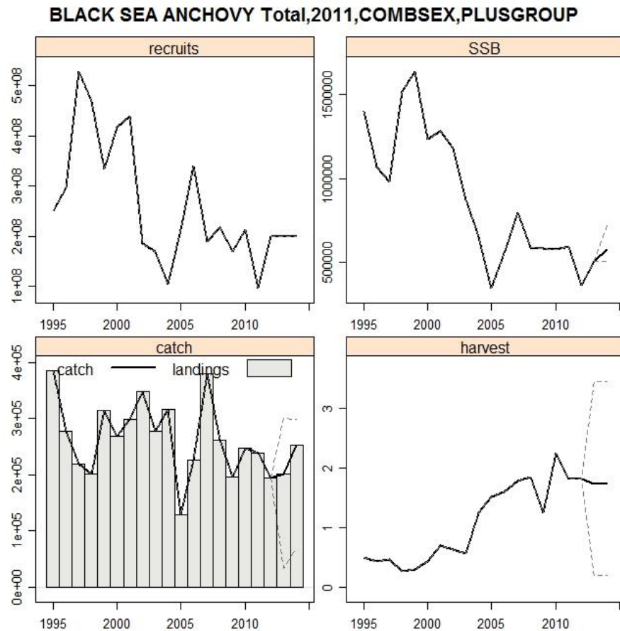
Fig. 31 – Short term prediction of the Black Sea anchovy stock parameters assuming status quo fishing in 2012 and F_{msy} in 2013
